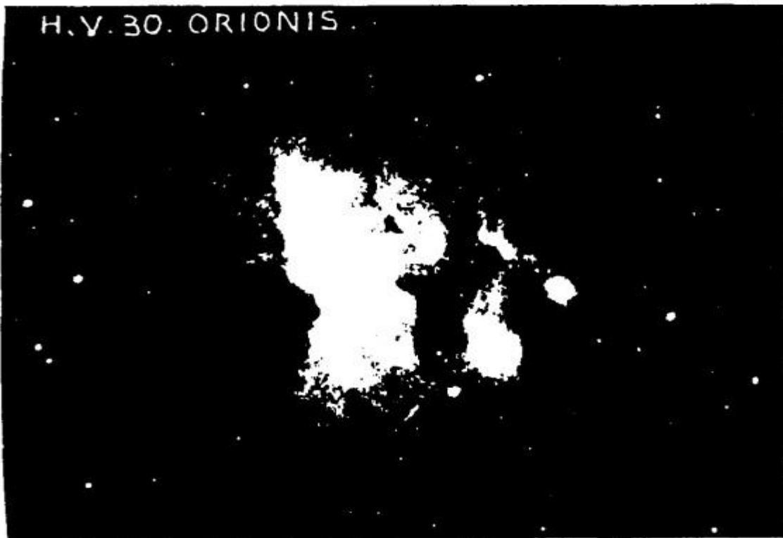
FIG. 43 Two exploding nebulas in Orion and Cephei which will send out fiery arms to form new star systems like the sun-spotted spiral pinwheels which are familiar objects in astronomical textbooks.
