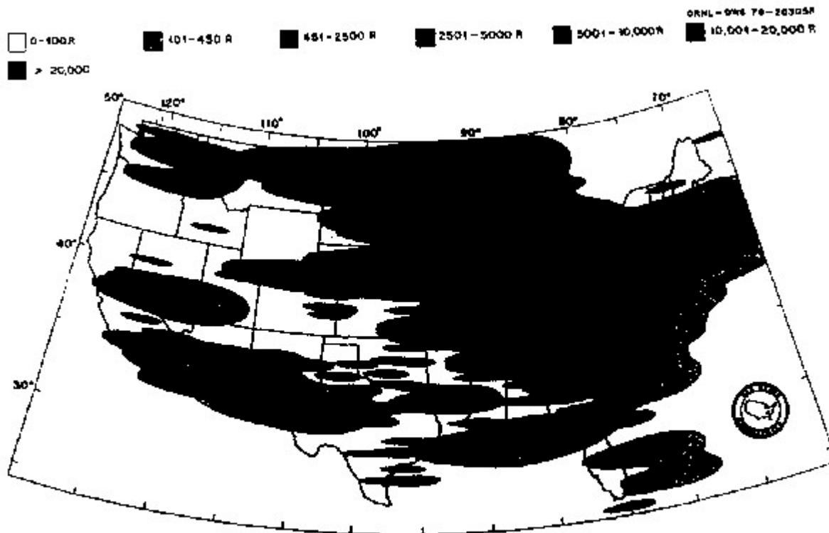
Fig. 4.1. Simplified fallout pattern showing total radiation dose that would be received by persons on the surface and in the open air for the entire 14 days following the surface burning of 5050 megatons on the targets indicated, if the winds of all directions blew continuously from the west at 25 mph.
