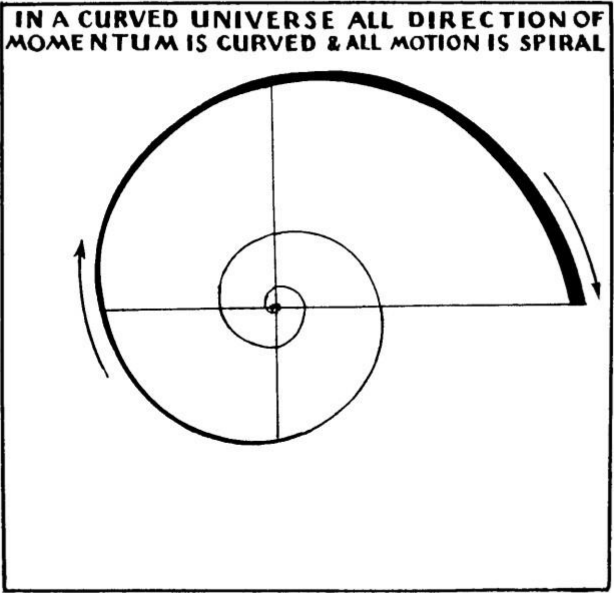
FIG. 47 Illustrating spiral principle in the starry heavens.
